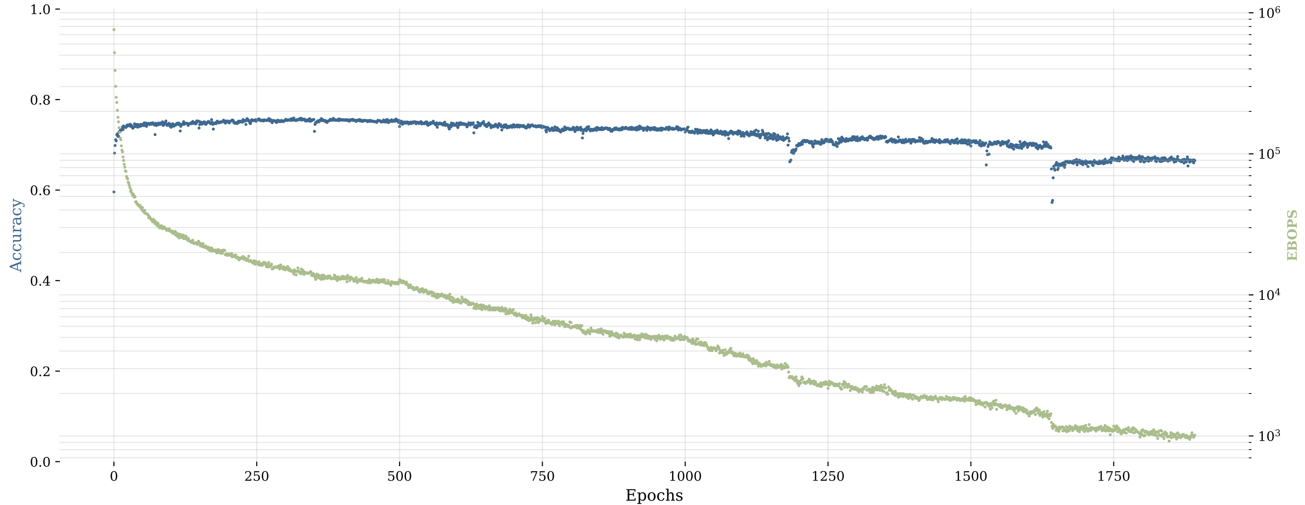
Pixel Splitting HGQ: Accuracy and EBOPS over Epochs
